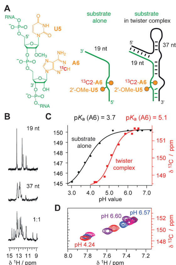
Figure 4. The adenine at the cleavage site of the twister ribozyme has a shifted pK a . A) Chemical structures of 13 C2-labeled A6-2'-OCH 3 -U5 (left) and cartoon of the strands used in the NMR experiments. B) Complex formation verified by 1 H NMR imino proton spectroscopy. C) Chemical shift changes of 13 C2-A6, with changes in the pH value derived from 1 J( 1 H, 13 C) HSQC spectra. The lines represent least-squares fits. [33] D) Exemplary 1 J( 1 H, 13 C) HSQC spectra of pH-dependent NMR experiments of 13 C2-A6 labeled twister. Conditions: c(RNA) = 0.5 mM; 100 mM KCl, 2 mM MgCl 2 , 10 mM Na cacodylate, H 2 O/D 2 O 9:1, 298 K.
